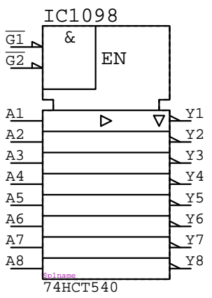
74HCT540 IC????
