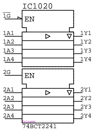
74BCT2241
