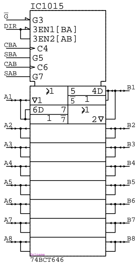
74BCT646
