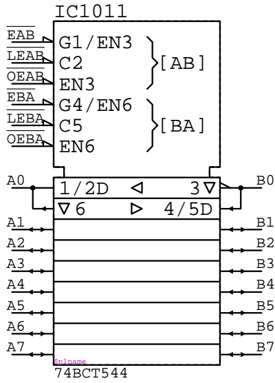
74BCT544
