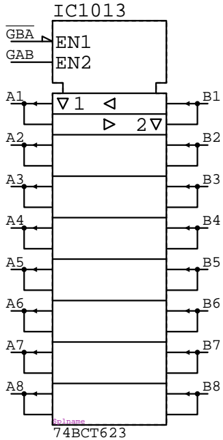
74BCT623
