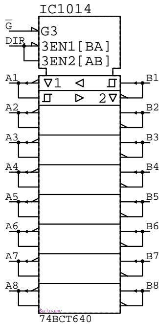
74BCT640
