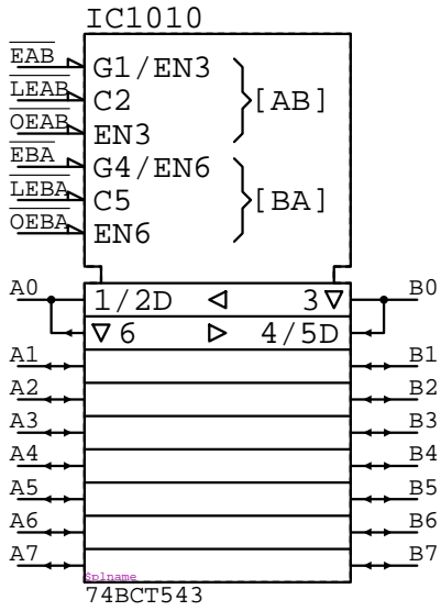
74BCT543
