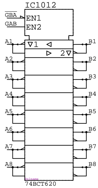
74BCT620
