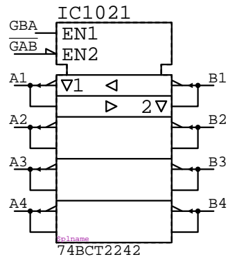
74BCT2242
