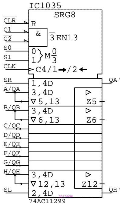
74AC11299 IC?????
