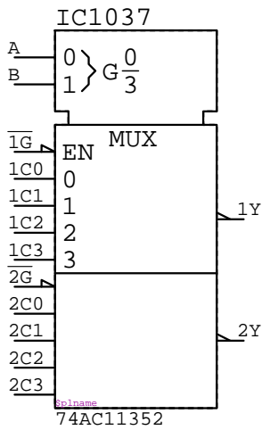
74AC11352 IC????
