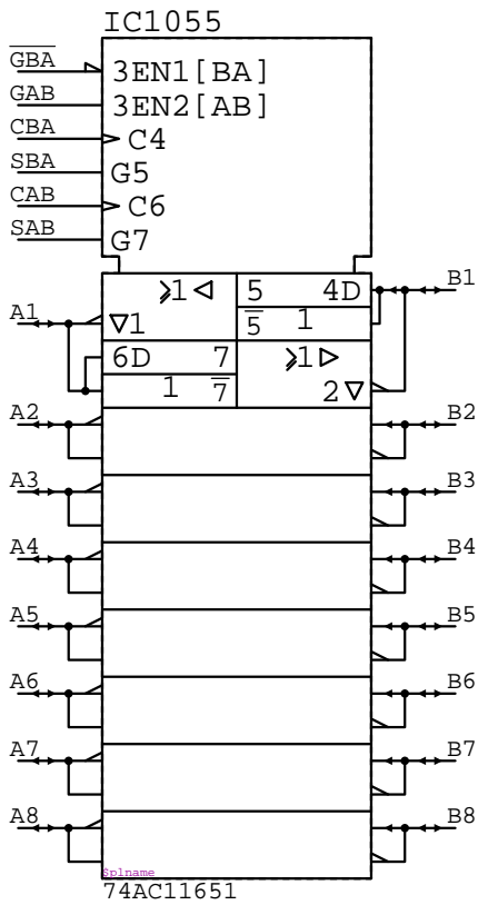
74AC11651
