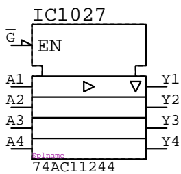
74AC11244 IC?????
