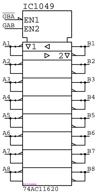
74AC11620 IC?????
