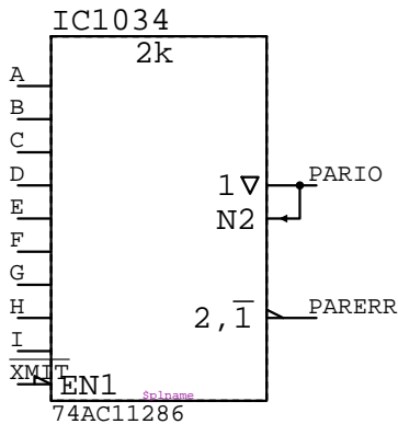
74AC11286 IC?????
