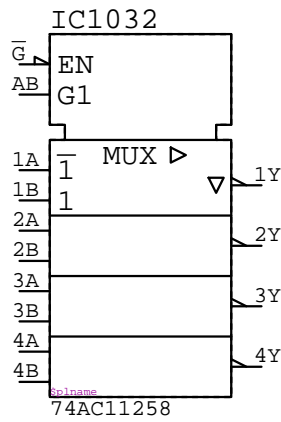
74AC11258 IC?????
