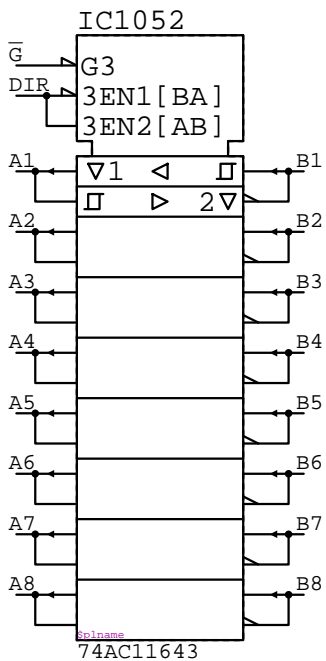
74AC11643 IC?????
