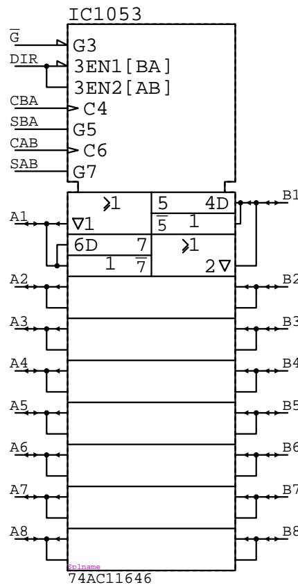
74AC11646 IC?????
