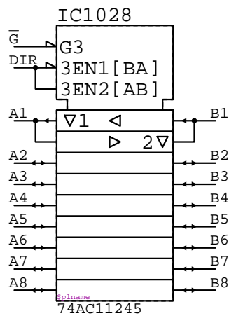
74AC11245 IC?????
