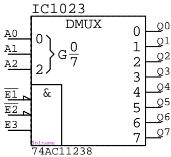
74AC11238 IC?????
