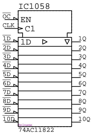
74AC11822
