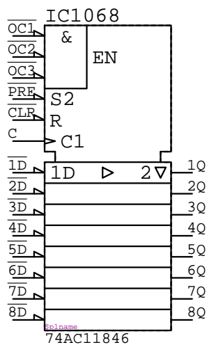
74AC11846
