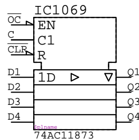
74AC11873
