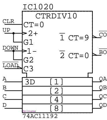
74AC11192 IC?????
