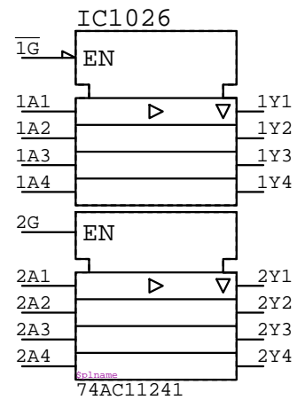
74AC11241 IC?????
