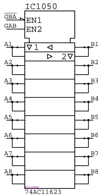
74AC11623 IC?????
