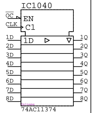
74AC11374 IC????
