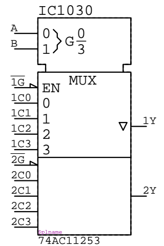
74AC11253 IC?????
