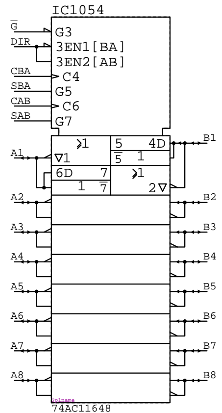
74AC11648 IC?????
