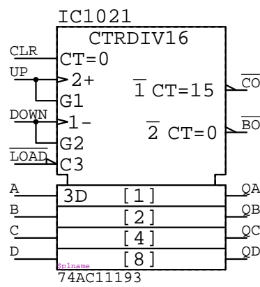
74AC11193 IC?????
