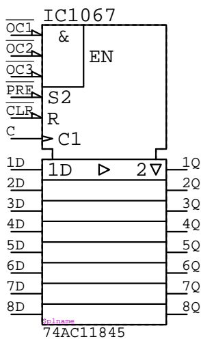
74AC11845
