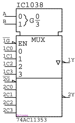
74AC11353 IC????
