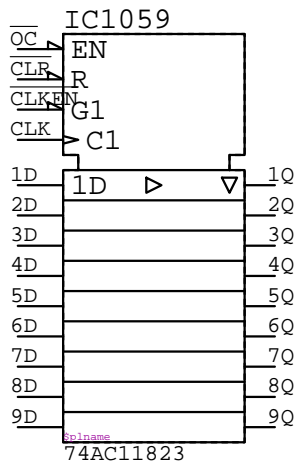
74AC11823
