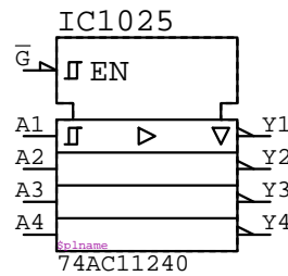
74AC11240 IC?????
