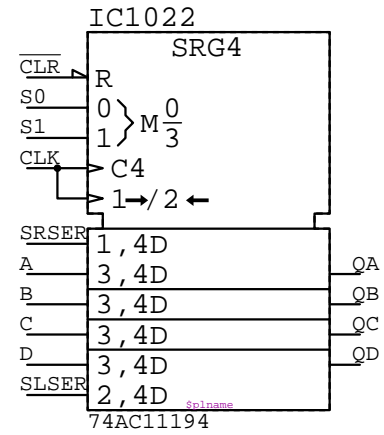
74AC11194 IC?????
