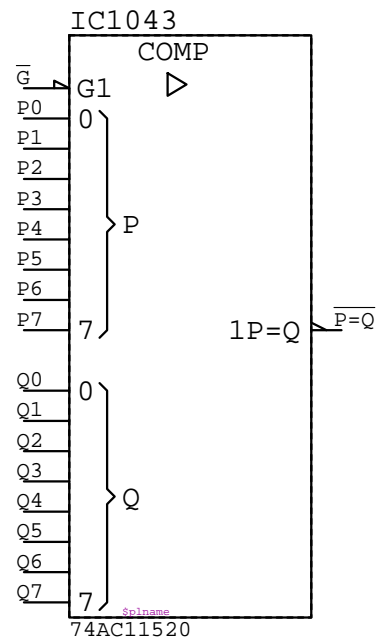
74AC11520 IC????
