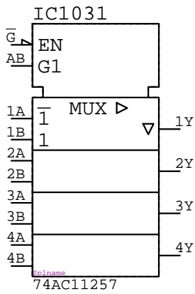
74AC11257 IC?????
