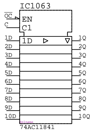
74AC11841
