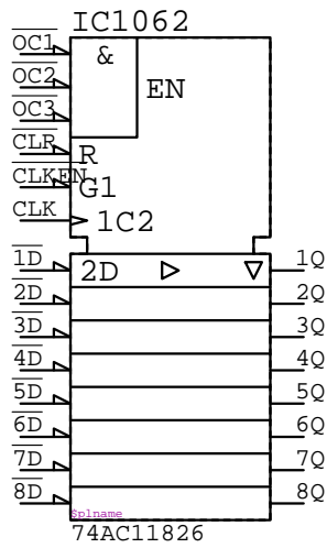
74AC11826
