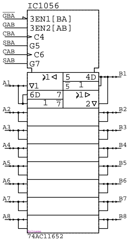
74AC11652
