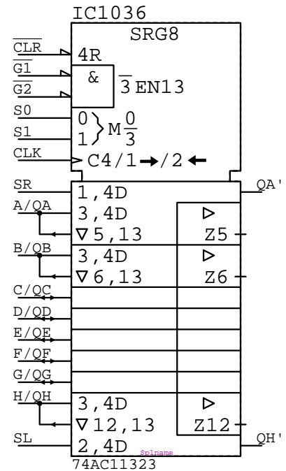
74AC11323 IC?????
