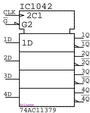
74AC11379 IC????
