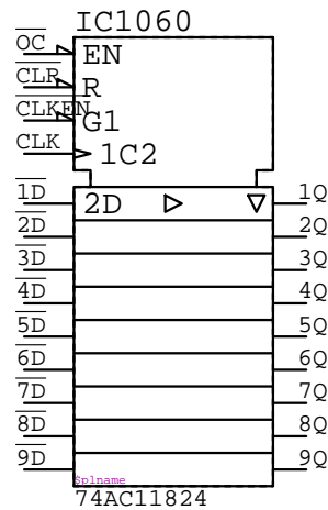
74AC11824
