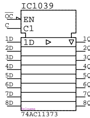
74AC11373 IC????
